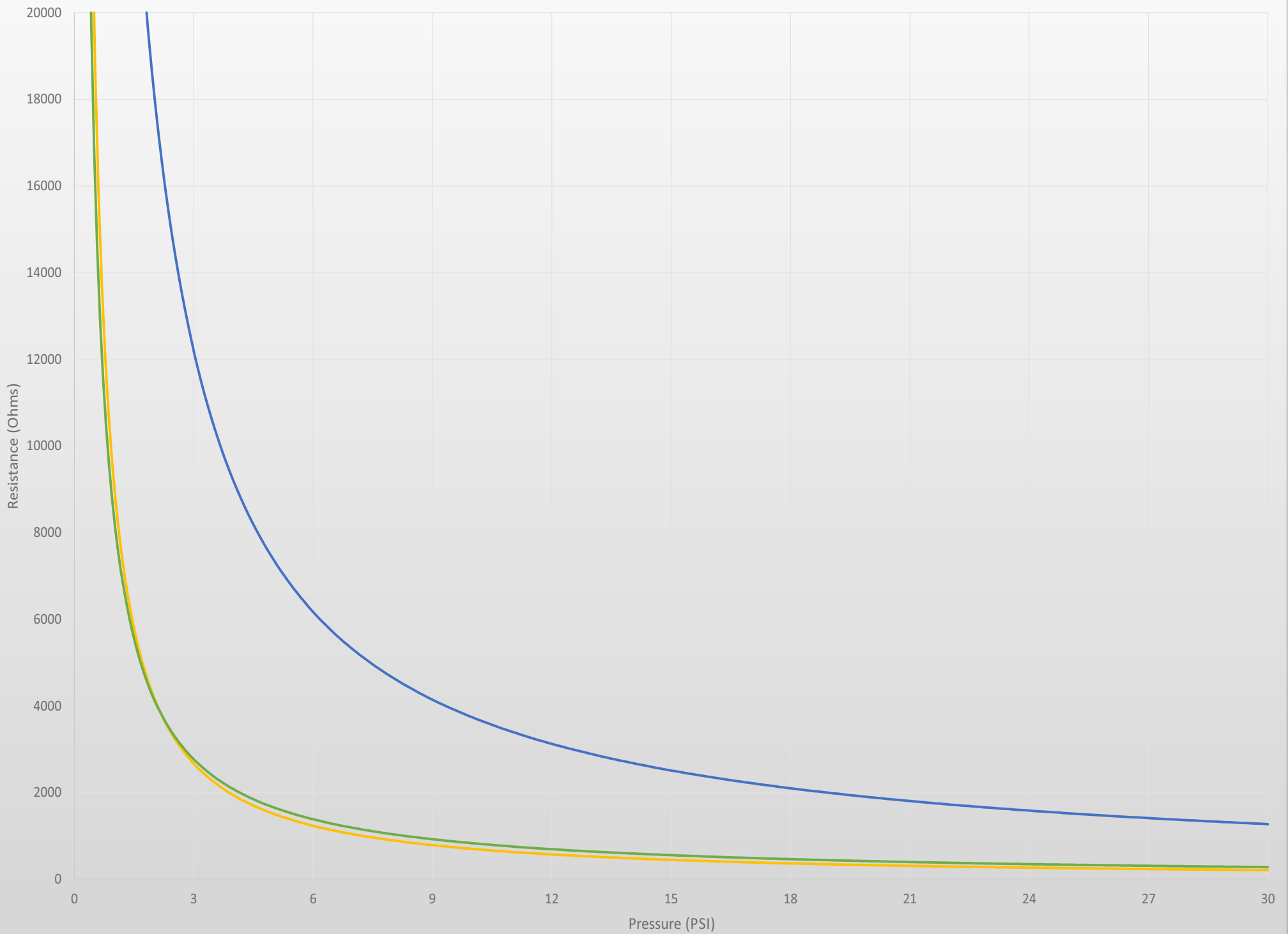
1/2" Thru Mode Sensor Responses
