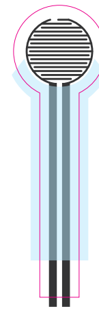
LOWER CIRCUIT (TOP SIDE) 1. CI-1001 CONDUCTIVE SILVER, 2. DI-7502 UV DIELECTRIC
