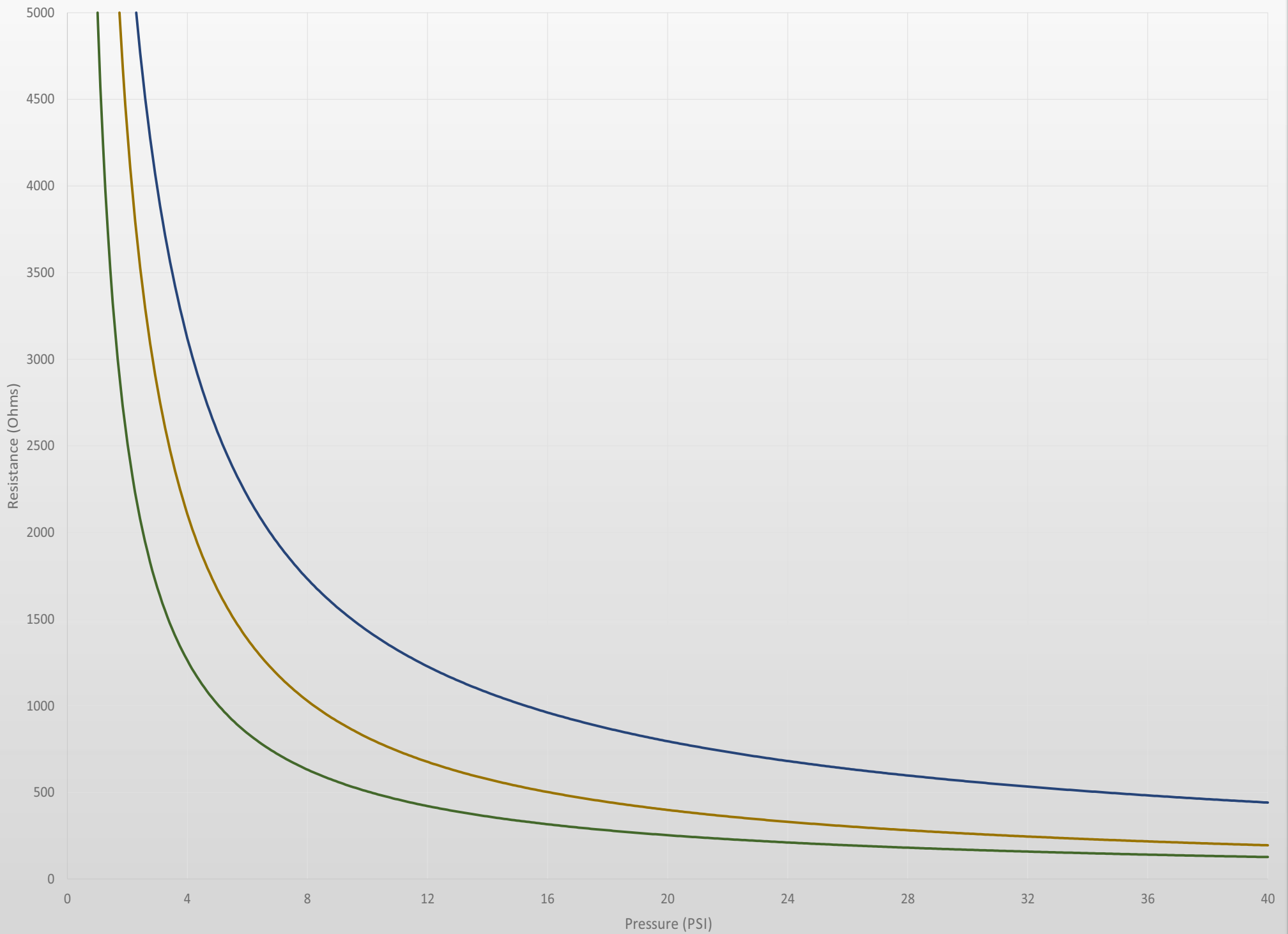
1" Thru Mode Sensor Responses
