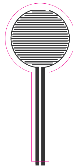
LOWER CIRCUIT (TOP SIDE) 1. CI-1001 CONDUCTIVE SILVER, 2. DI-7502 UV DIELECTRIC
