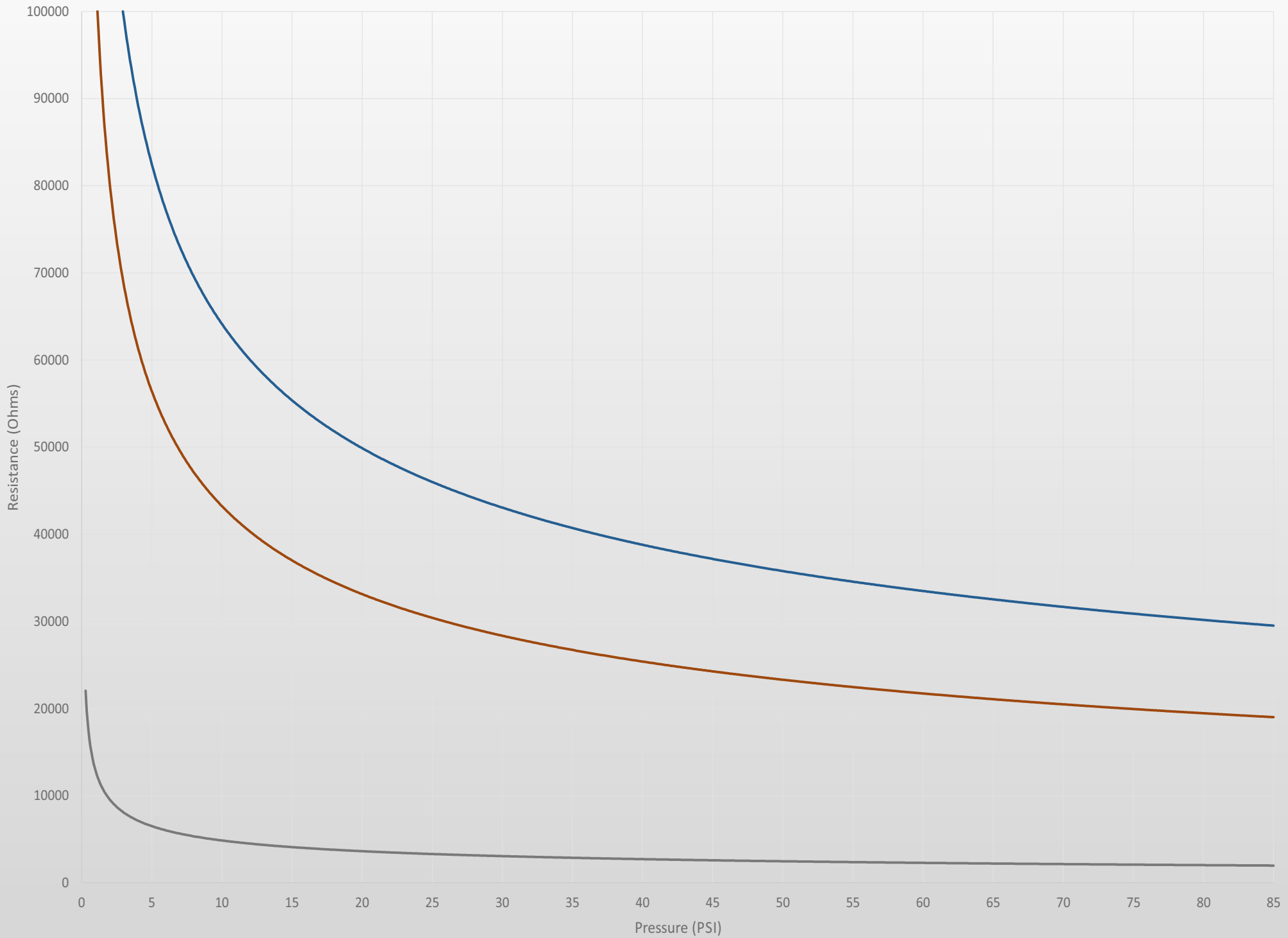
1" Shunt Mode Sensor Response
